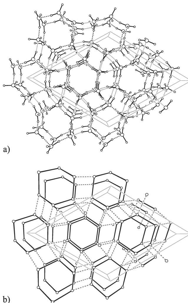
Figure 3. (a) View of the crystal packing in rhombohedral \text{Me}_3\text{In} along the hexagonal c -axis showing intermolecular \text{In}\cdots\text{C} contacts (dashed and dotted lines). (b) View of the 3D network formed by \text{Me}_3\text{In} molecules as pseudo-tetrahedral nodes ( \text{Me}_3\text{In} molecules are represented by indium atoms and the longer \text{In}\cdots\text{C}\text{--In} bridges are shown by dashed lines).
