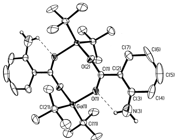
Fig. 1 Molecular structure of [(t\text{Bu})_2\text{Ga}(\mu\text{-O}_2\text{CC}_6\text{H}_4\text{-2-NH}_2)]_2 ( 2 ). Thermal ellipsoids are shown at the 30% level, and hydrogen atoms bound to carbon are omitted for clarity. Hydrogen bonding interactions are denoted by a dashed line.
