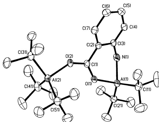
Fig. 5 Molecular structure of (t\text{Bu})_2\text{Al}(\mu\text{-O}_2\text{CC}_6\text{H}_4\text{-2-NH}_2)\text{Al}(t\text{Bu})_3 ( 5 ). Thermal ellipsoids are shown at the 30% level, and hydrogen atoms are omitted for clarity.
