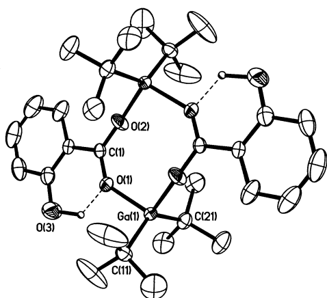
Fig. 2 Molecular structure of [(t\text{Bu})_2\text{Ga}(\mu\text{-O}_2\text{CC}_6\text{H}_4\text{-2-OH})]_2 ( 3 ). Thermal ellipsoids are shown at the 30% level, and hydrogen atoms bound to carbon are omitted for clarity. Hydrogen bonding interactions are denoted by a dashed line.
