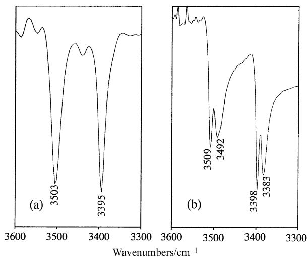
Fig. 4 IR spectra of [(t\text{Bu})_2\text{Ga}(\mu\text{-O}_2\text{CC}_6\text{H}_4\text{-2-NH}_2)_2] in toluene solution (a) and the solid state (b) showing the presence of discrete hydrogen bonded and the non-hydrogen bonded N–H groups.
