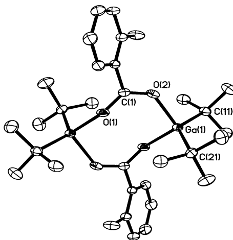
Fig. 3 Molecular structure of [(t\text{Bu})_2\text{Ga}(\mu\text{-O}_2\text{CC}_6\text{H}_4\text{-2-Me})]_2 ( 4 ). Thermal ellipsoids are shown at the 30% level, and hydrogen atoms are omitted for clarity.
